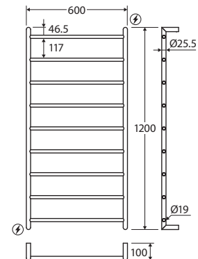
⚡ Wiring Positions
